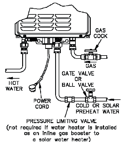
Gas Water Heater Cold (or Solar Preheat) and Hot Water and Gas Connection Details
